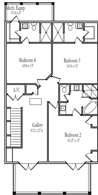
Second Floor Plan N.T.S
