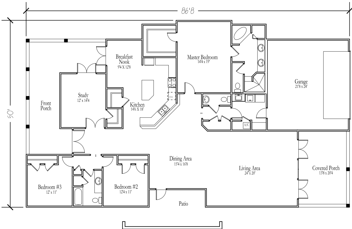
Floor Plan
