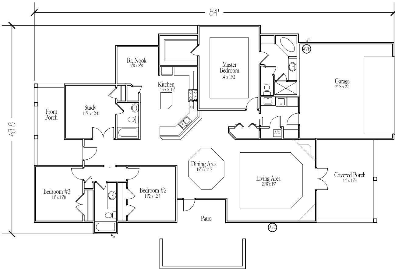
Floor Plan
