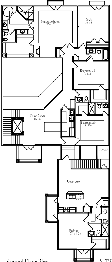
Second Floor Plan N.T.S
