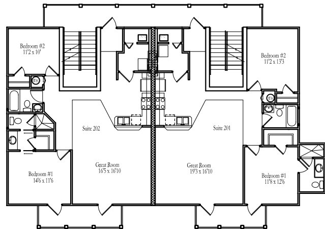
Second Floor Plan N.T.S
