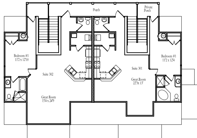
Third Floor Plan N.T.S
