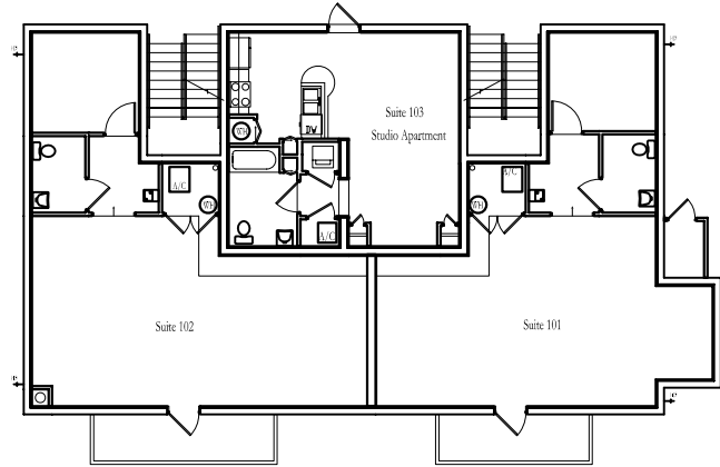
First Floor Plan N.T.S
