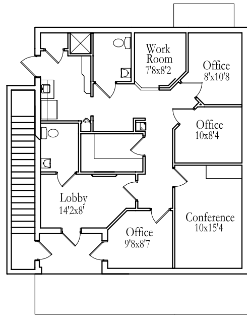
Second Floor Plan N.T.S
