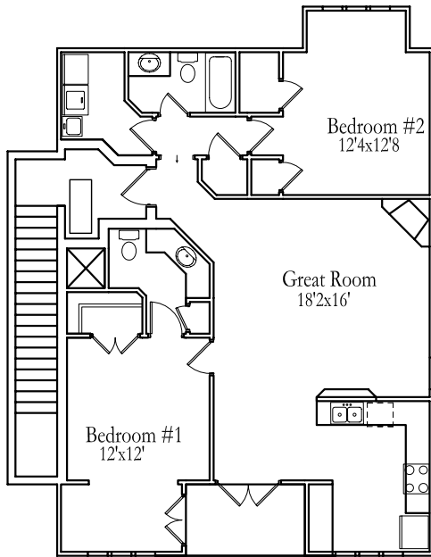
First Floor Plan N.T.S
