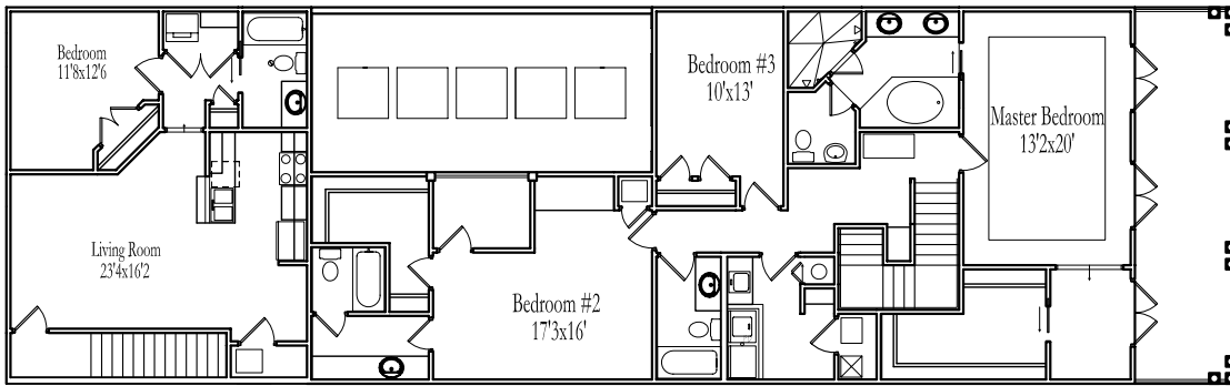
Second Floor Plan N.T.S
